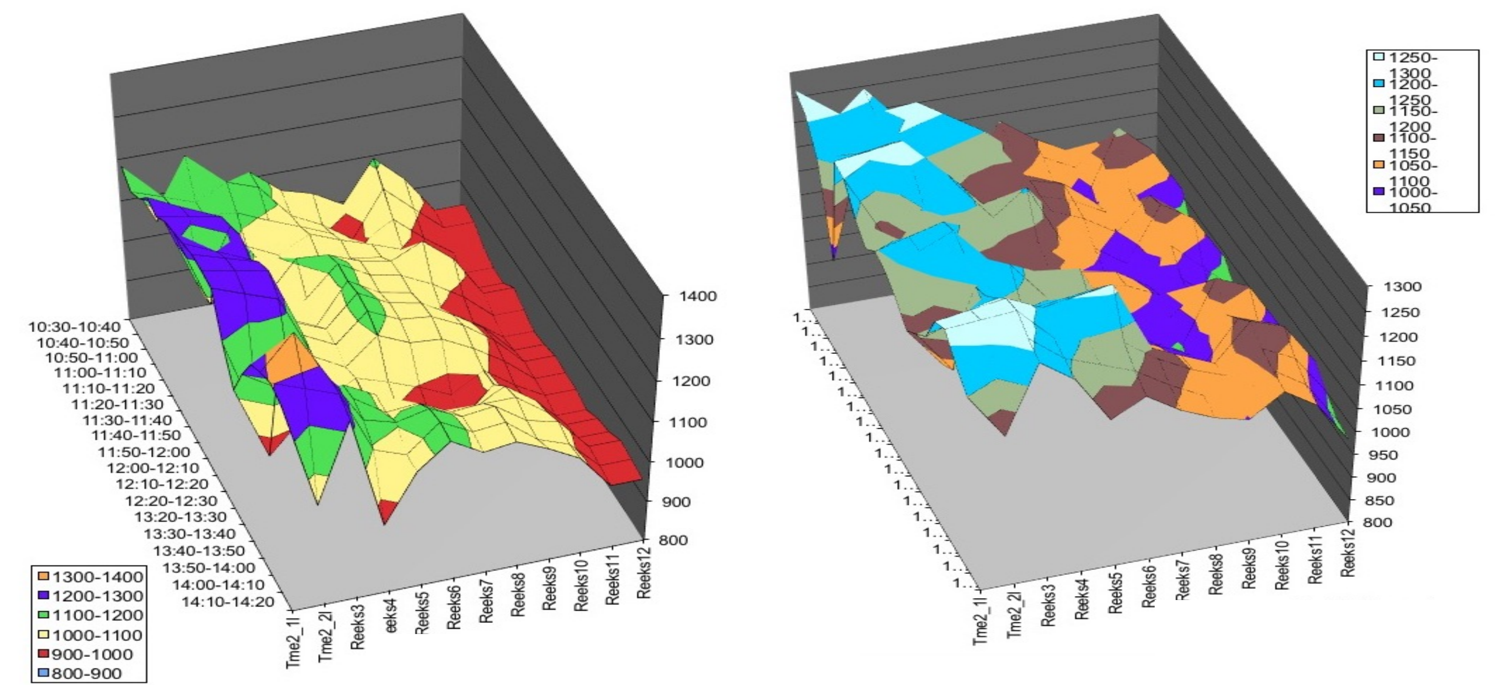
Figure 2: Part and full load temperature in PostCombustion Zone (18 m)
