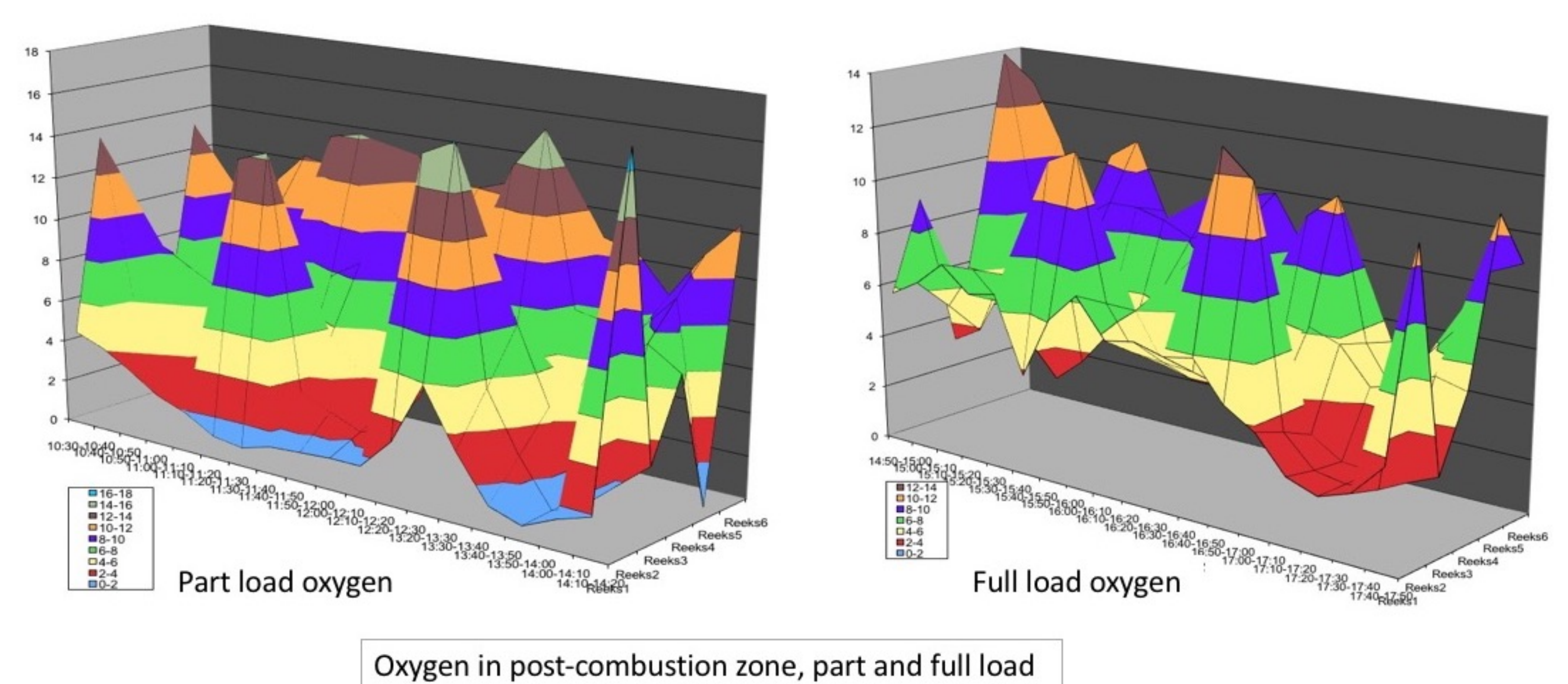
Figure 3: Part and full load oxygen in PostCombustion Zone (18 m)
